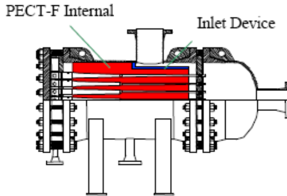
Figure 7. Conventional deoiling hydrocyclone vessel equipped with PECT technology [7]
