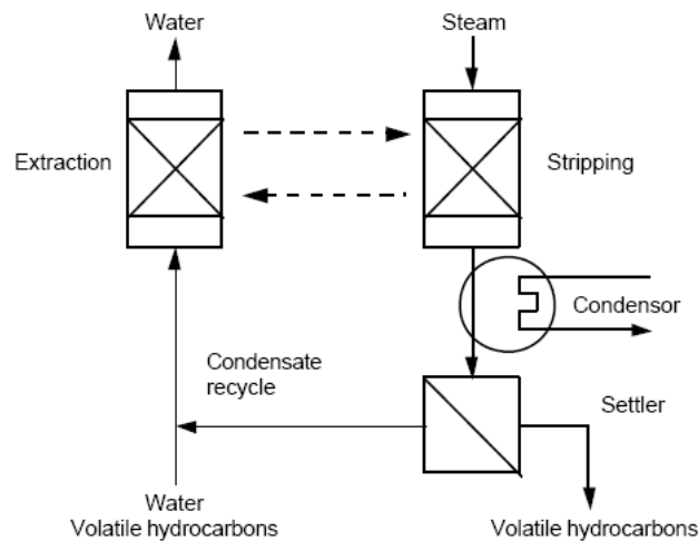
Figure 12. MPPE extraction/ stripping system [27]
