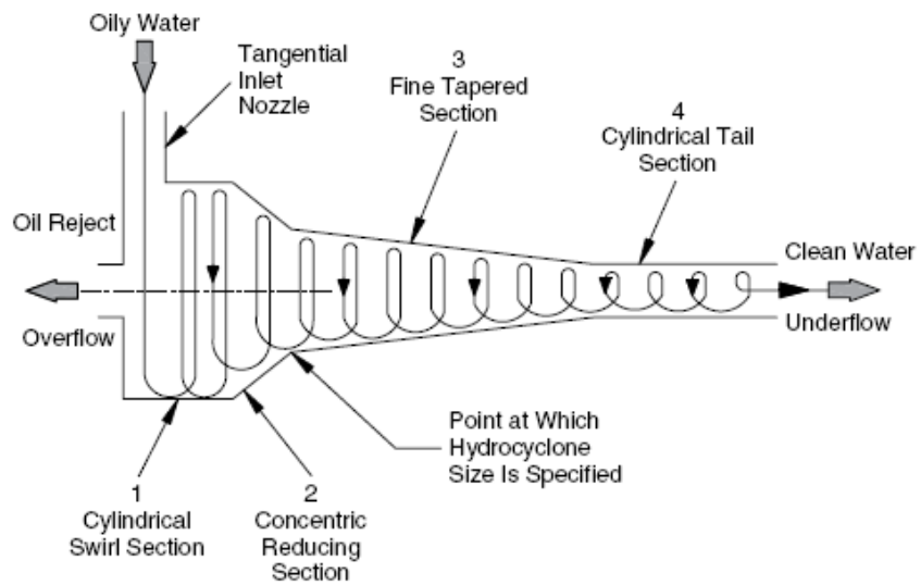
Figure 9. Principles of operation of a hydrocyclone: 1) cylindrical swirl chamber 2)concentric reducing section 3) fine tapered section 4) a cylindrical tail section [4]
