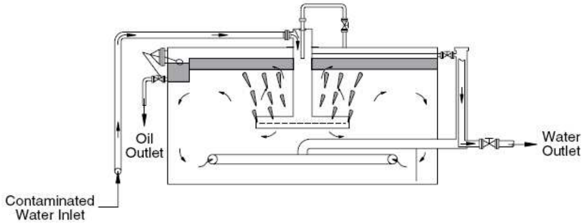
Figure 3. Schematic of a skimmer tank [4]
