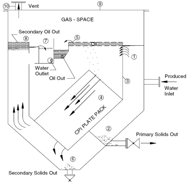
Figure 5. Schematic showing flow pattern of a typical down-flow CPI design [4]
