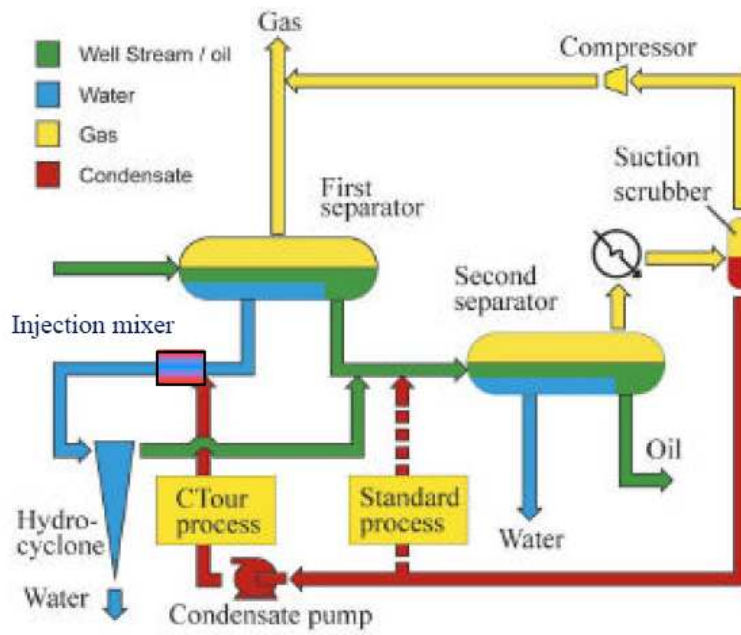
Figure 11. Flow diagram of the CTour process [11]
