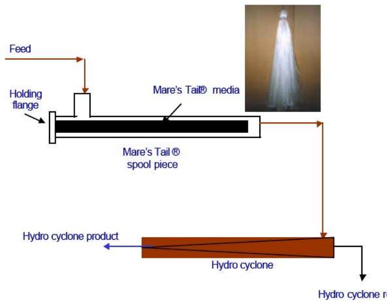
Figure 8. Principle of operation of Mare's Tail [11]
